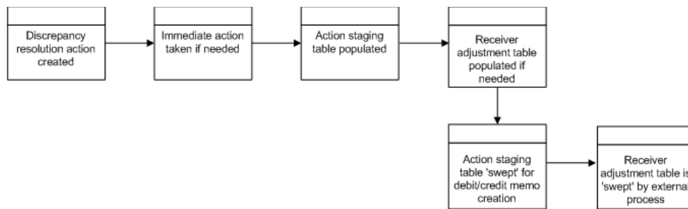
Figure 7-3 ReIM Reason Code Action Rollup Flow
