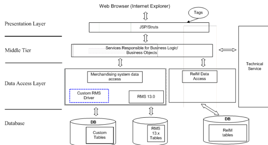
Figure 3–1 ReIM Layered Architecture
