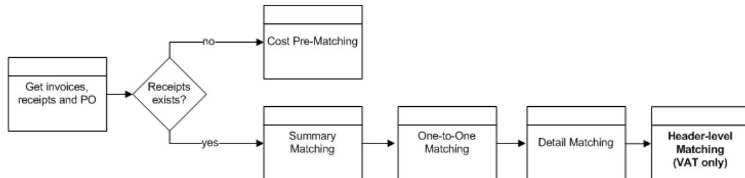
Figure 7-1 ReIM iauto-match flow
