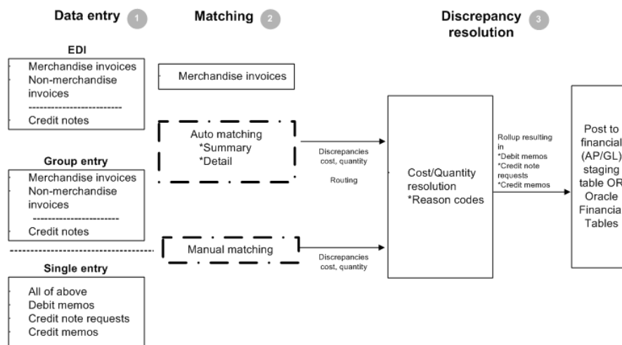
Figure 4–2 High-level view of the invoice and credit note matching process
