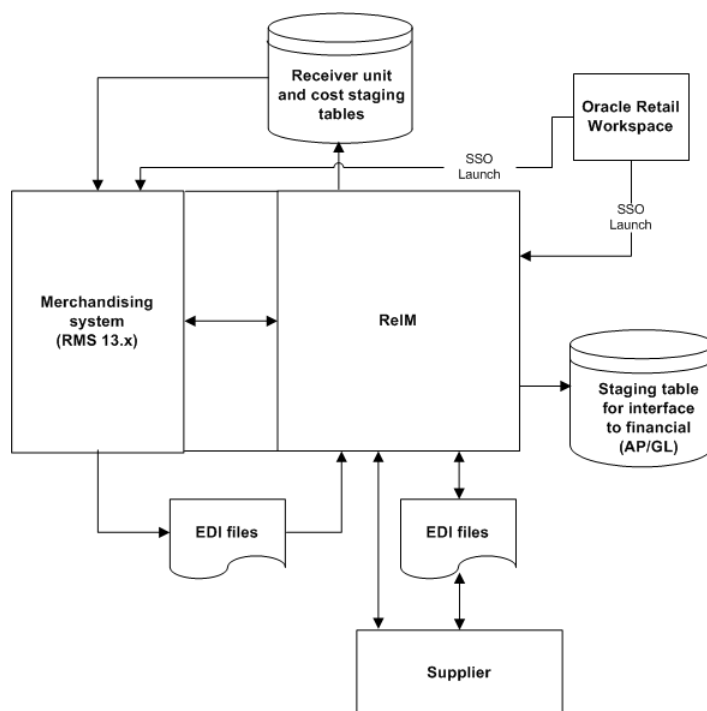
Figure 4–1 ReIM Dataflow across the Enterprise
